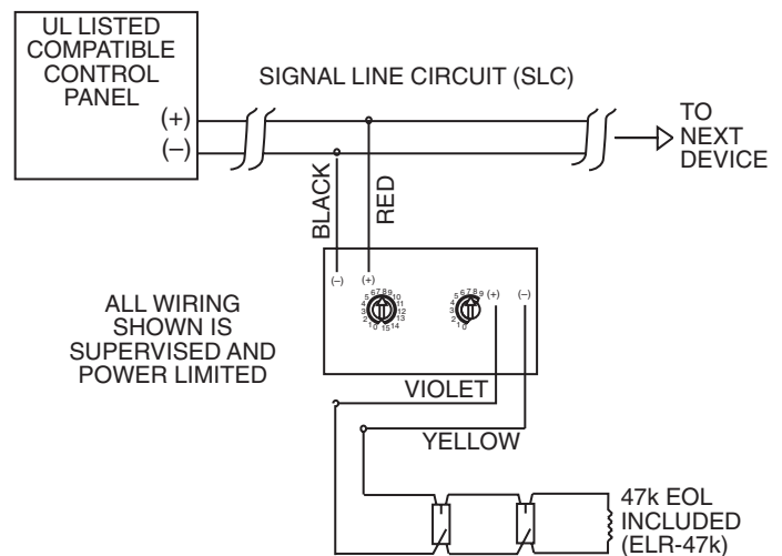
FIGURE 2. TYPICAL 2-WIRE STYLE B INITIATING DEVICE CIRCUIT CONFIGURATION:
