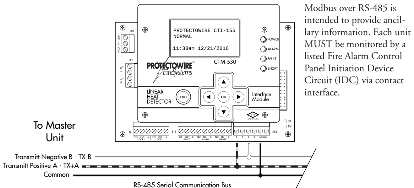
Wiring Diagram - Figure 1
