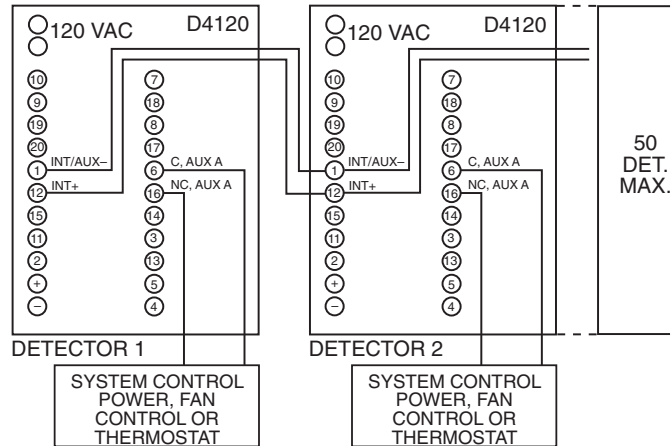
FIGURE 8. MULTIPLE FAN SHUTDOWN (INTERCONNECTION OF D4120'S):
